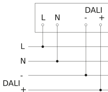
Master circuit diagram
